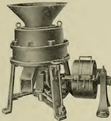
FIG. 152.—Paint-grinding Mill.
